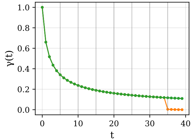
Ackley-20D
