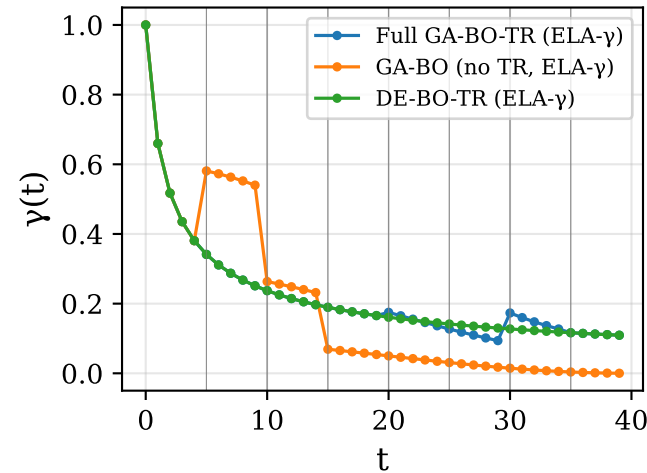
Ackley-5D
