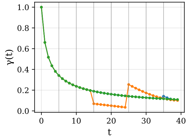
Rastrigin-10D
